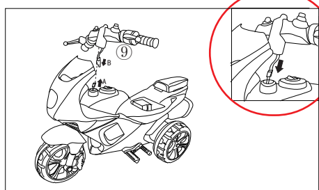
(5). Refer to the picture, plug the "B" plugs on the handle and the "A" plugs on the body with the motorcycle body firmly.
