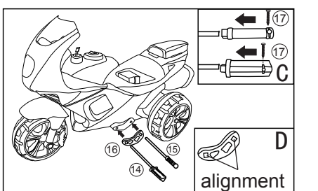
(4). Refer the picture, separately insert the pedal shaft (14) and gear shaft (15) through the limit films(16) then into the 2 holes on the motorcycle( aim at the square hold which showed on Pic D). After through the other side of the motorcycle, the axle will be covered a limit films and another pedal sets and gear sets. And fixed by 2 pcs of round heads self-tapping screws of 4*12 (Note: should assemble the right and left body symmetrically).
