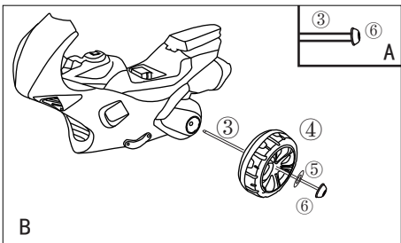
2. Refer the picture, Knock the wheelcap(6) with hammer and let it combine the rear axle then put a 10mm flat gasket (5). (Note: the flat gasket will be covered on the arrow shows the position which in the middle of the wheel and wheelcap), then covered by a wheel (4), then insert the hold of the gear box which loaded in the rear body of the motorcycle,the rear axle will be out from the other side of the motorcycle,then put another wheel (4) and also put a 10 mm gasket (5), at last,put the wheelcap (6), then lock the rear wheel.
